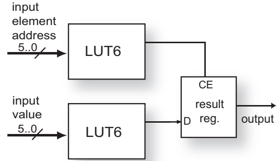
Fig. 7. LUT6-based FU implementation.
