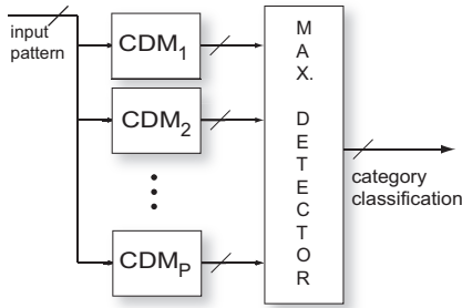
Fig. 1. A high-level overview of the on-chip EHW system.
